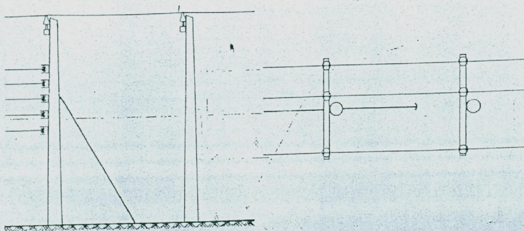
SECONDARY DEAD END THROUGH PRIMARY
