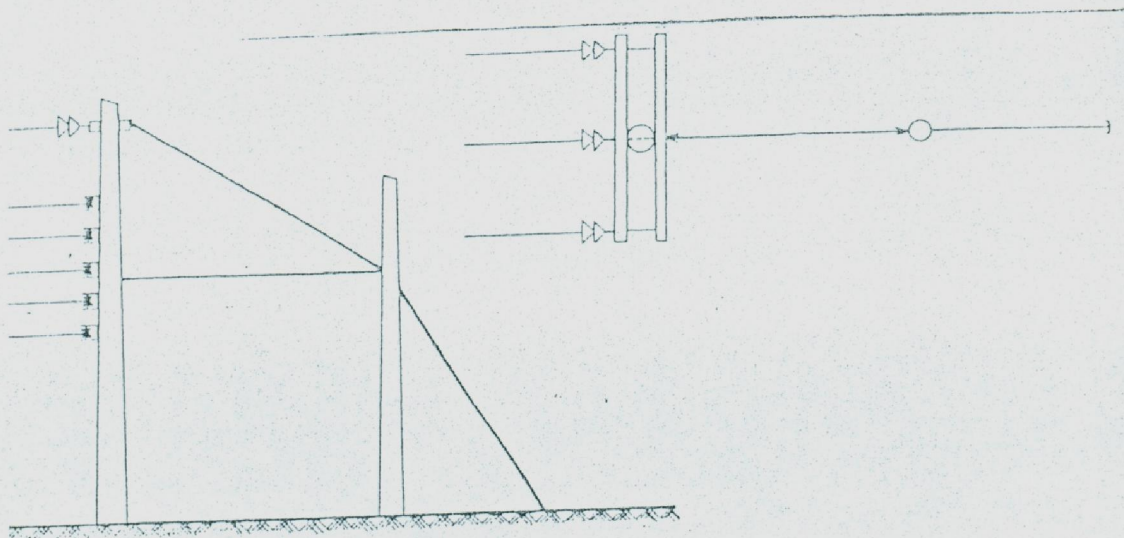
PRIMARY & SECONDARY DEAD END WITH STUB GUY
