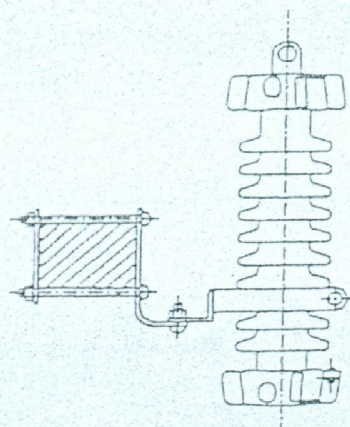
Fig 3-a Side mounting , 90° bracket
