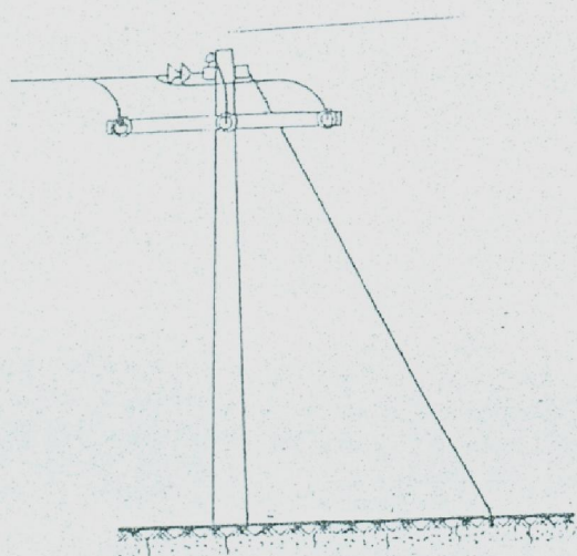
PRIMARY, TWO DOWN GUYS FOR LARGE ANGLES & HIGHER TENSIONS
