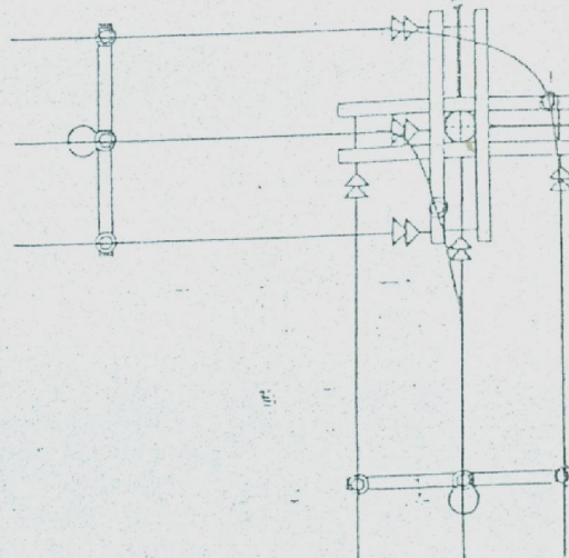
PRIMARY, TWO DOWN GUYS FOR LARGE ANGLES & HIGHER TENSIONS
